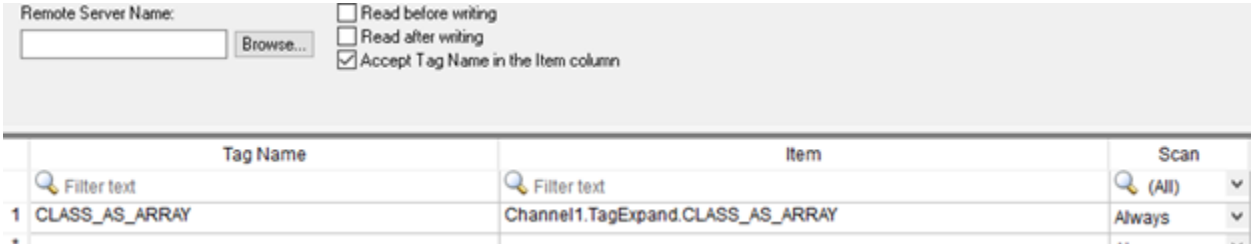
Associating the OPC groups with the array of classes
