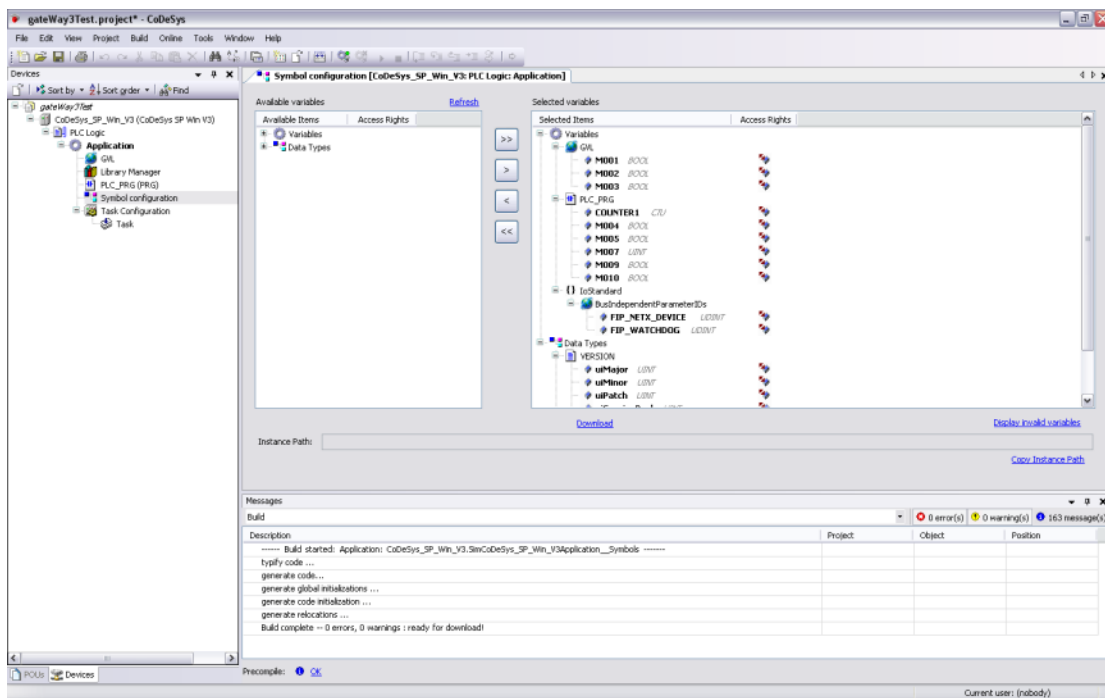
Moving variables in the Symbol Configuration object
